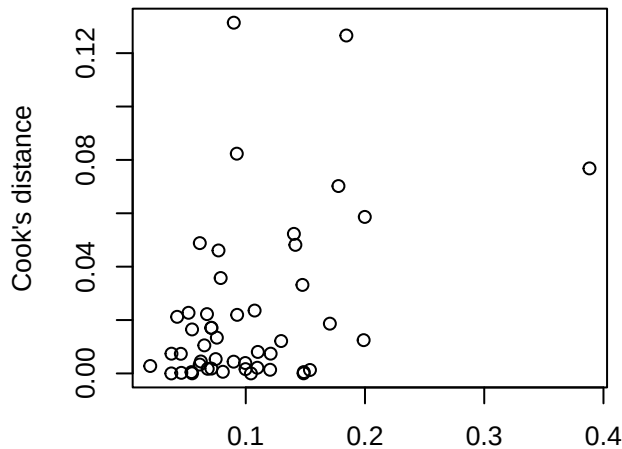
Cook's dist vs Leverage
